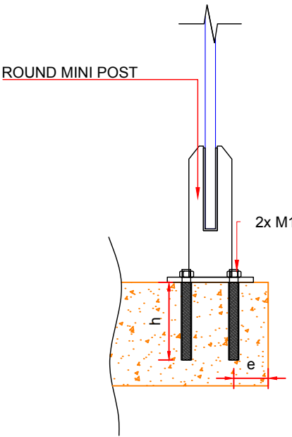
CONNECTION TO CONCRETE
