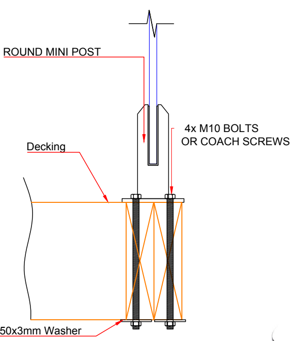
CONNECTION TO TIMBER
