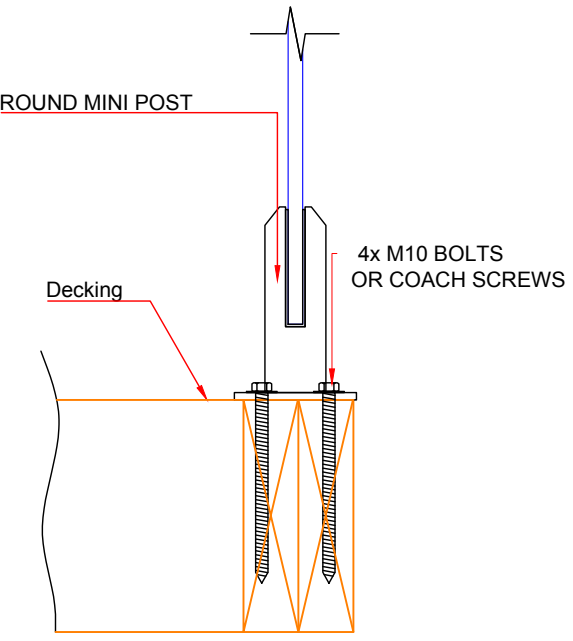
CONNECTION TO TIMBER
