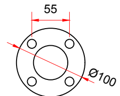
BASE PLATE LAYOUT
